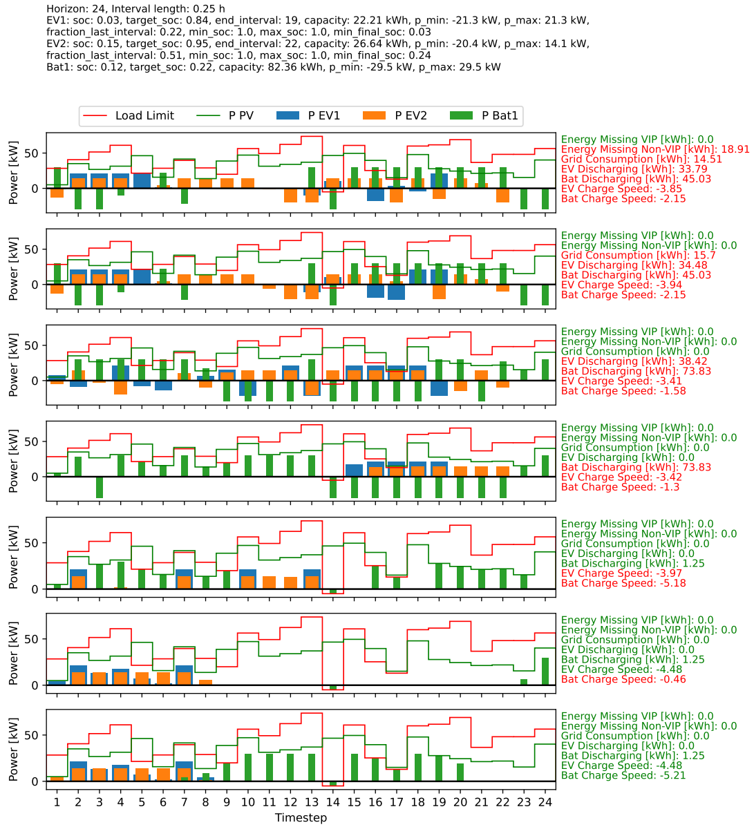
Fig. 6: Illustration of a use case showing inputs and schedules resulting from the optimizations with respect to the different objectives of the hierarchy. Objectives shown in green are considered (optimized), those in red not.
