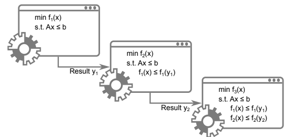
Fig. 4: Illustration of hierarchical optimization with three objectives.
