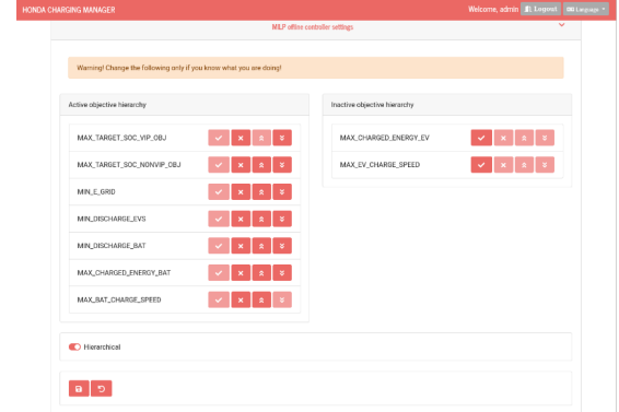
Fig. 5: Screenshot of the charging manager configuration user interface allowing the setting of the objective hierarchy.
