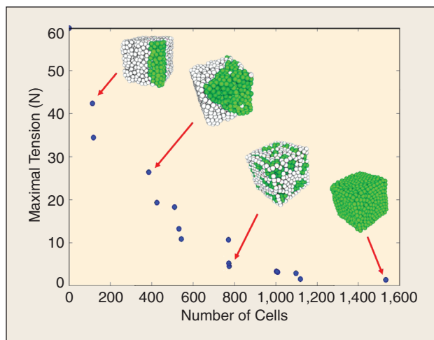
FIGURE 11 Pareto-optimal solutions for lightweight stable structures obtained from a cellular growth model.
