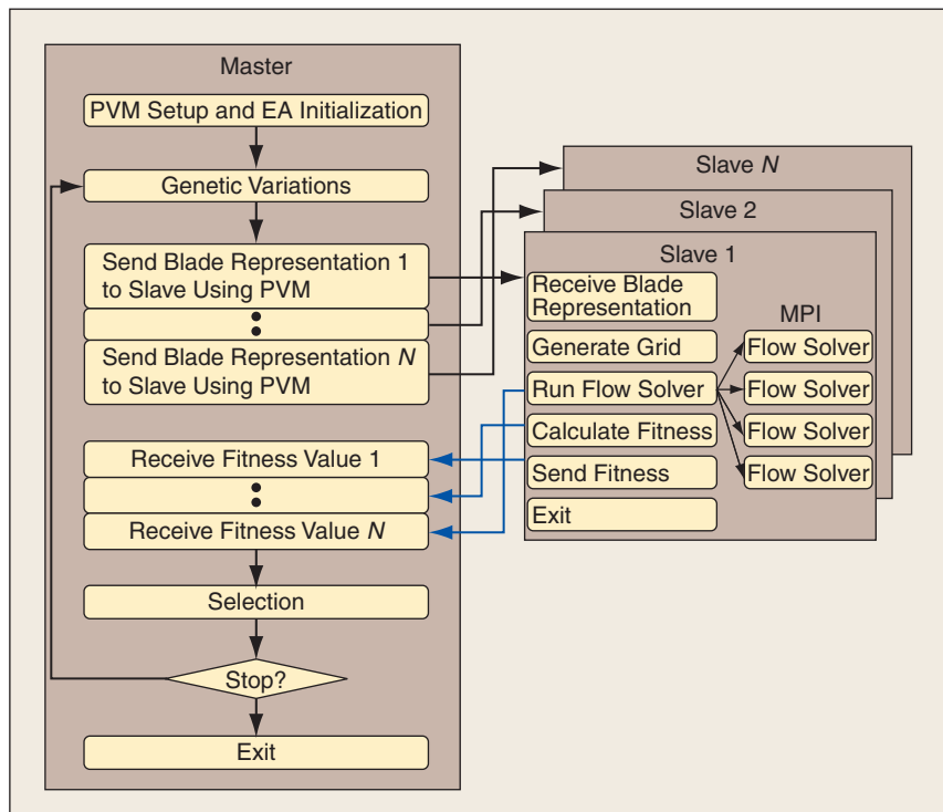
FIGURE 7 A computing architecture with both population level and individual level of parallelization.
