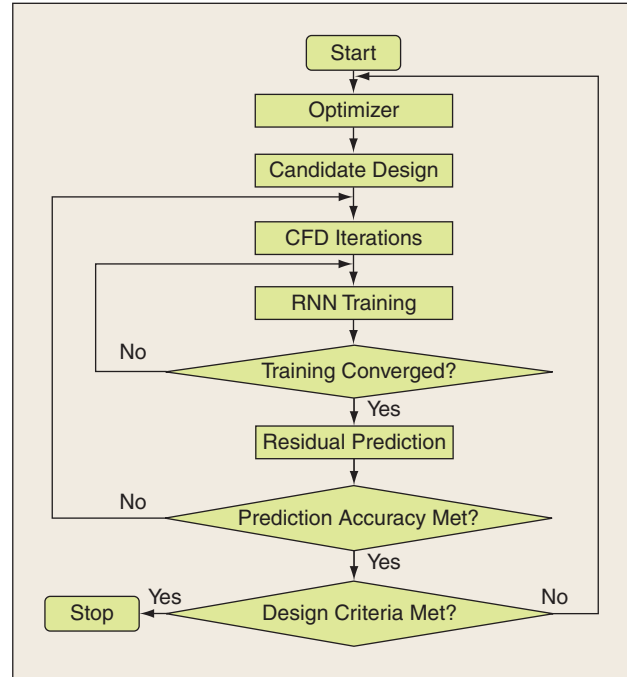
FIGURE 6 A diagram showing how recurrent neural networks can be used for predicting results in CFD iterations.
