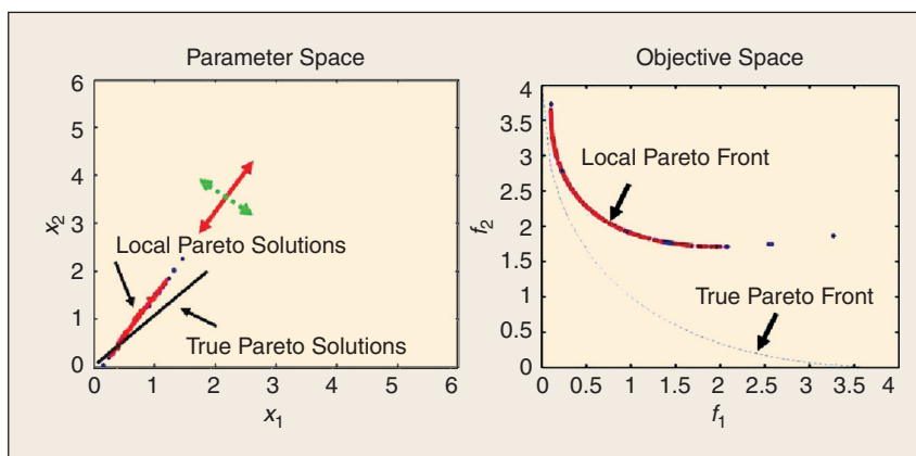
FIGURE 2 Pseudo local Pareto front introduced by the BNDX on the 30-D Schaffer function.
