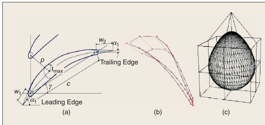
FIGURE 3 Three typical geometry representations. (a) Parametrized representation, (b) NURBS, (c) FFD.
