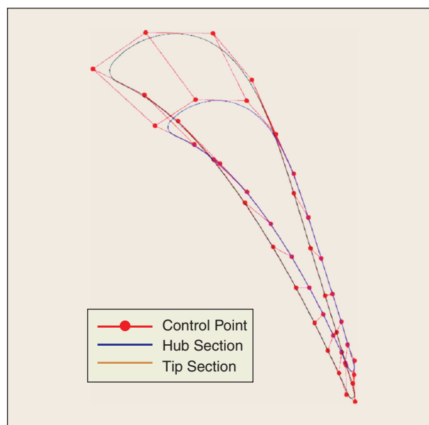
FIGURE 9 NURBS representation of a 3D turbine blade of a gas turbine.
