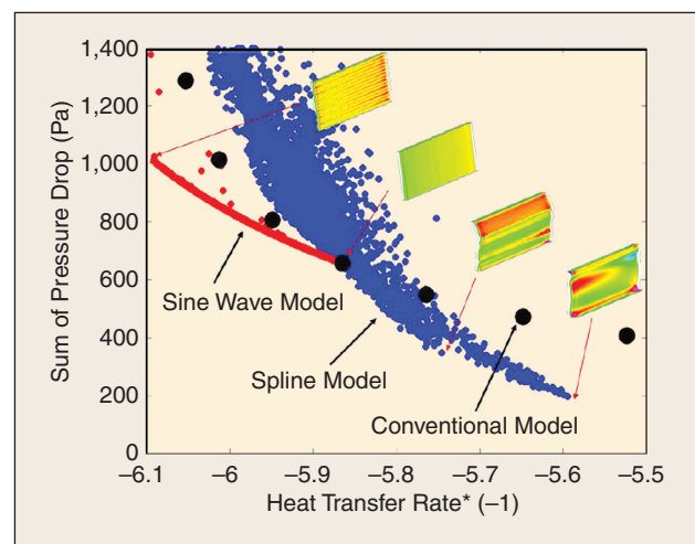
FIGURE 4 Obtained solutions using different geometry representations in an evolutionary optimization of a micro heat exchanger.
