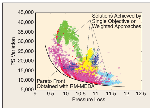
FIGURE 10 Results from the 3D design optimization as represented by NURBS in Figure 9.
