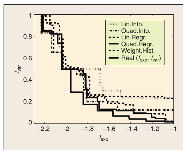
FIGURE 12 Pareto fronts obtained from the real fitness function and various surrogates.
