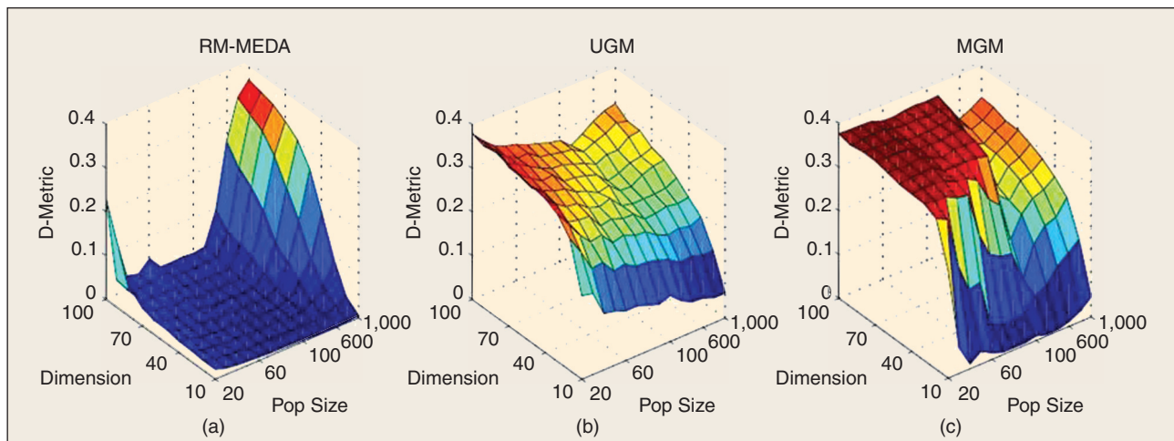
FIGURE 8 Scalability of three MOEAs on the test problem ZDT2.2, whose design parameters are nonlinearly correlated. (a) RM-MEDA. (b) UGM. (c) MGM.
