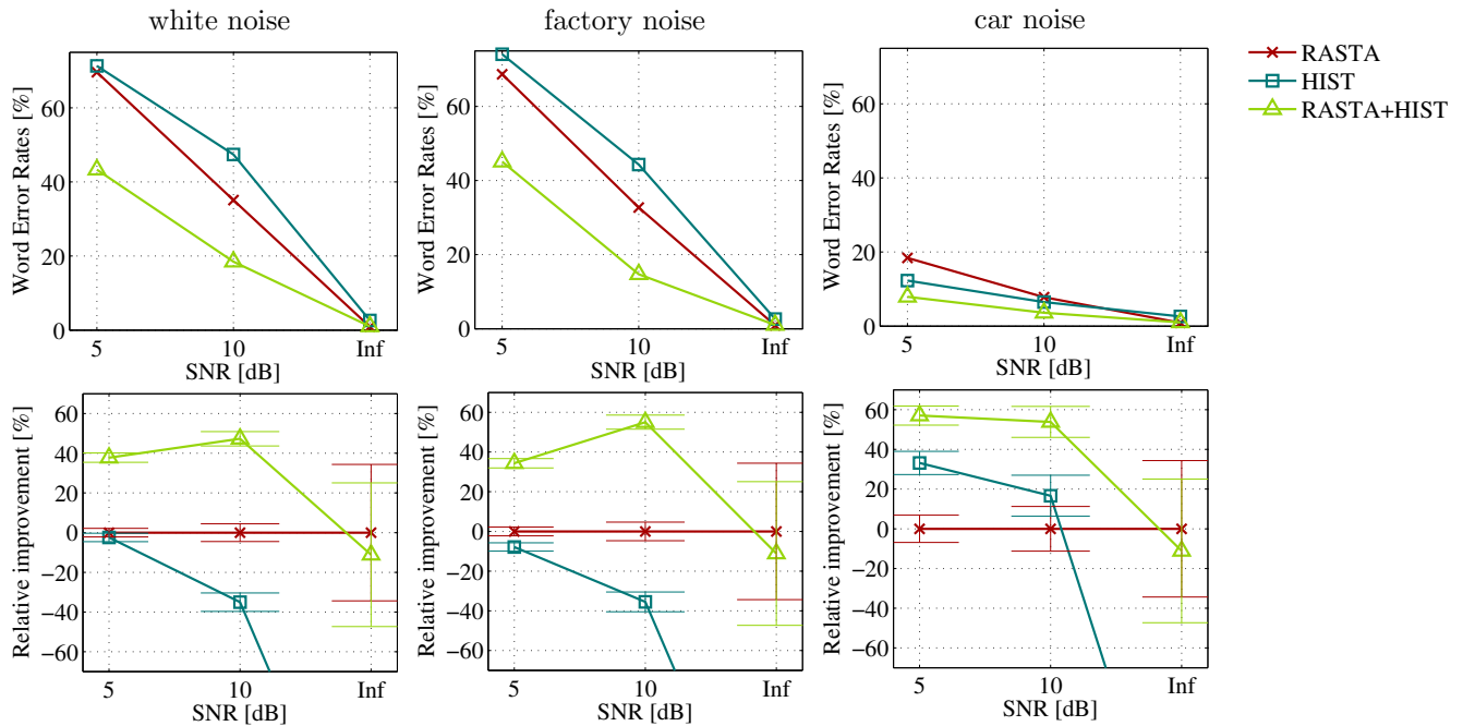
Figure 3: Recognition scores obtained for RASTA-PLP , HIST , and combined RASTA-PLP -HIST features on the complete TIDigits dataset. Noise type added and SNR level are indicated in the plots. The upper part shows the absolute errors, the lower part the errors relative to those obtained using only RASTA-PLP features. The bars in the lower part indicate the 95% confidence interval.
