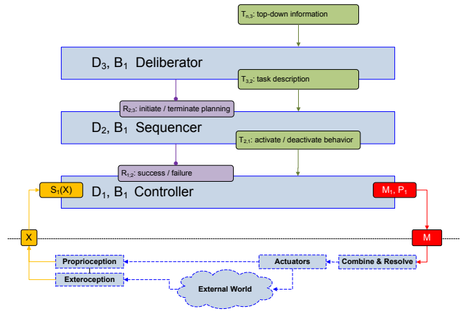
Fig. 5. Three Layer Architecture formulated in SYSTEMATICA.
