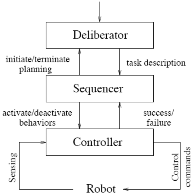
Fig. 4. Schema of Three Layer Architectures, taken from [27]
