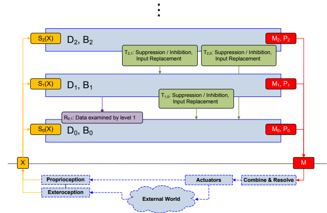
Fig. 3. Subsumption architecture formulated in SYSTEMATICA.
