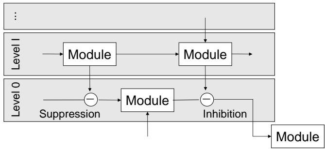
Fig. 2. Schema of subsumption architectures, drawing after [21]
