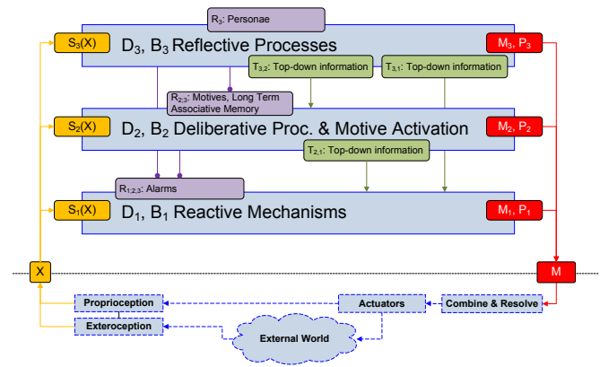
Fig. 7. HCOGAff Architecture formulated in SYSTEMATICA.
