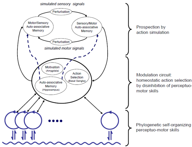
Fig. 8. Schematics of the iCub cognitive architecture, taken from [32]
