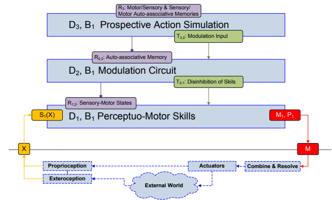
Fig. 9. The ICUB architecture formulated in SYSTEMATICA.
