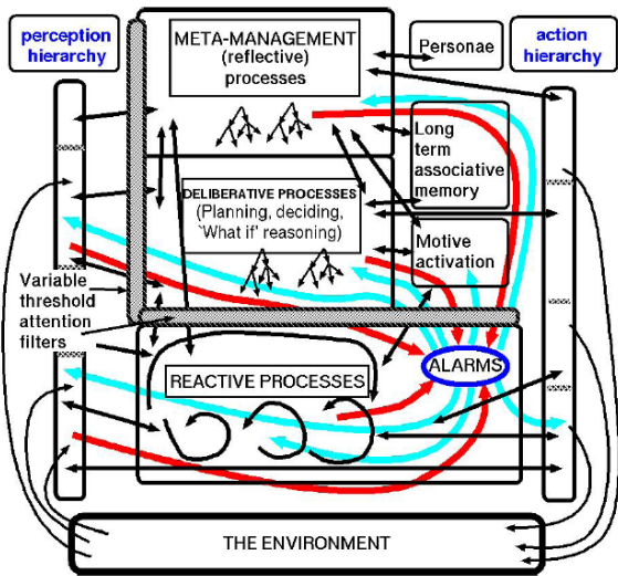
Fig. 6. Schematics of HCOGAff, taken from [31]
