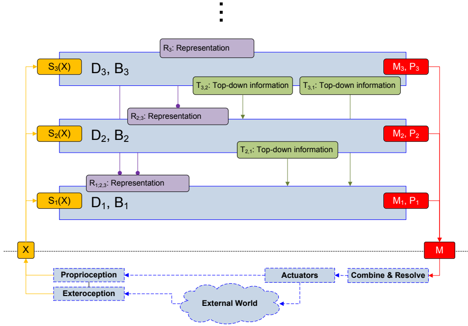
Fig. 1. Generic example of a SYSTEMATICA schematic showing a system with three layers.
